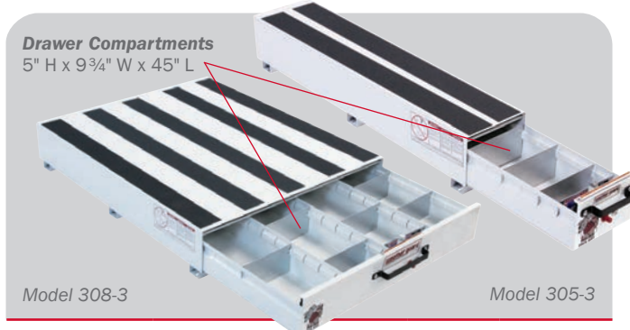
9½" High x 48" Long Drawer Units
