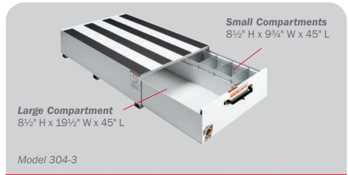
Extra Wide Compartment 48" Long Drawer Unit
